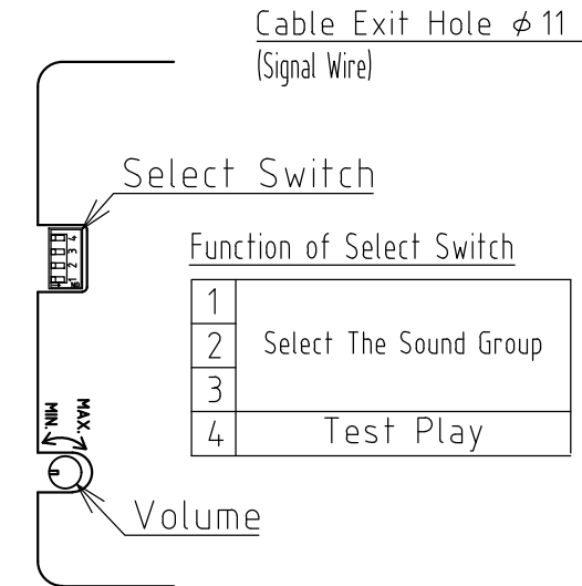
View 'A'
